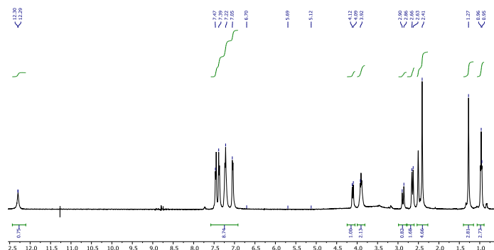
Figure 4. 1H NMR spectra of compound (4b)
