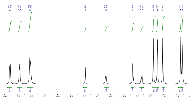
Figure 1. 1 H NMR spectra of compound (3b)
